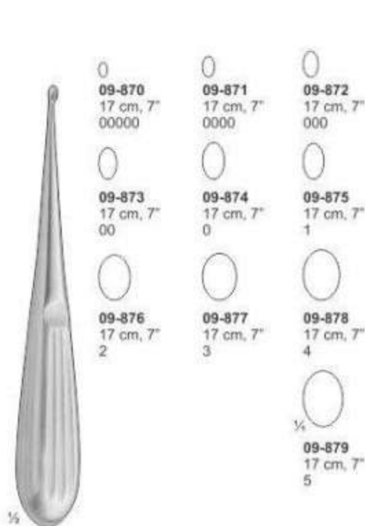
SPRATT / HOLLOW HANDLE
